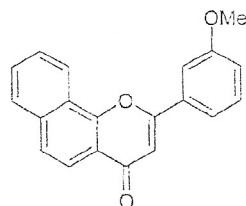
Chromatogram 3'-Methoxy-alpha-naphthoflavone D:\promonence\Data\2012\OCT-2012\071012H.lcd
