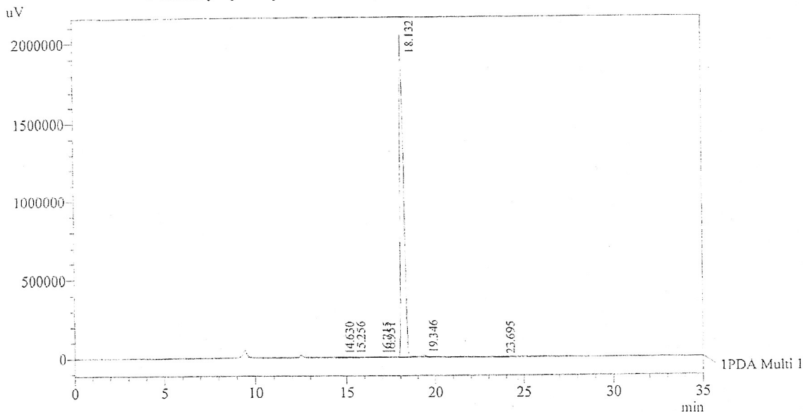
Chromatogram 3'-Methoxy-alpha-naphthoflavone D:\promonence\Data\2012\OCT-2012\071012H.lcd
